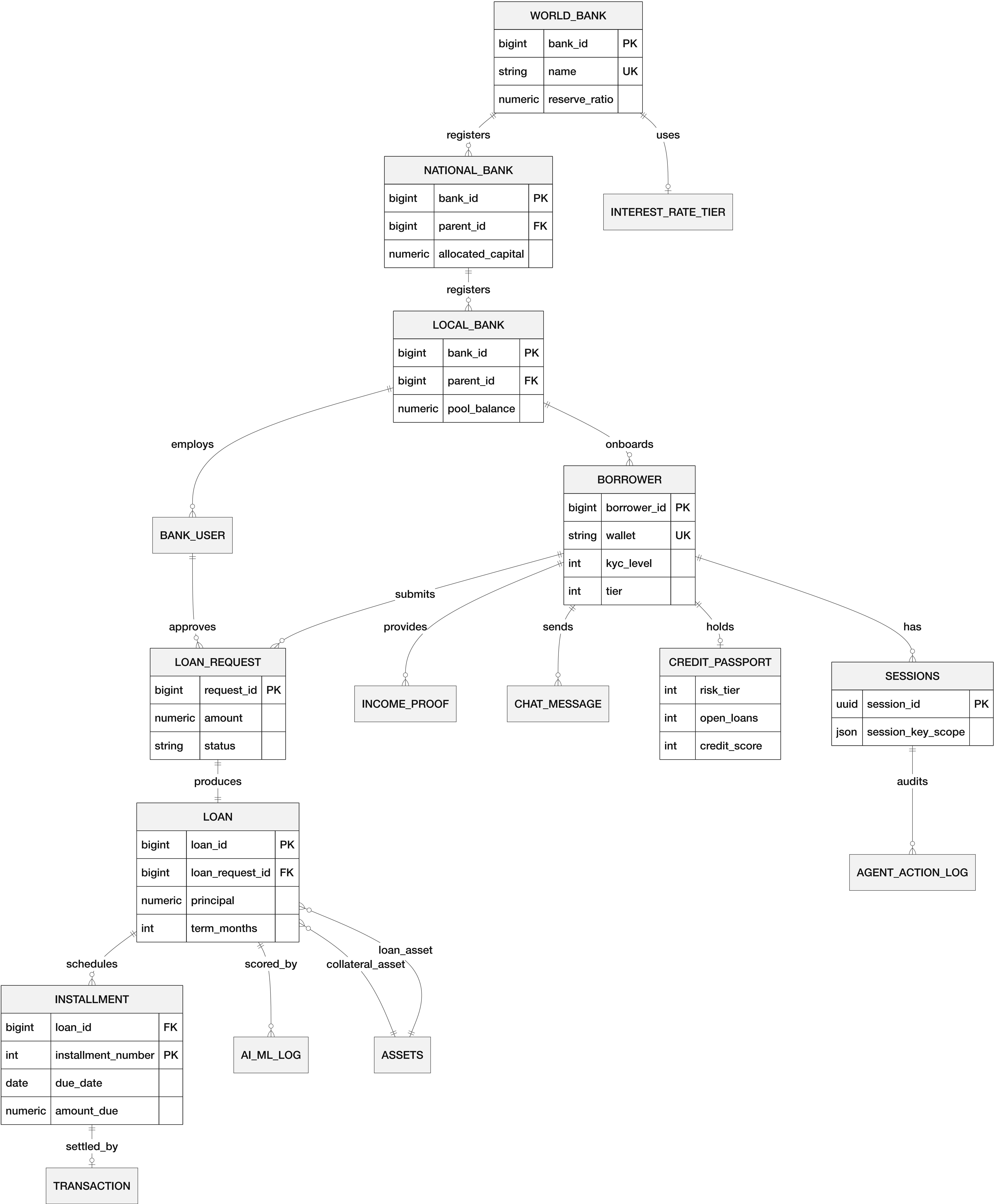
Core ERD - Lending, Governance, and Agent Session Entities
